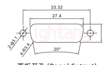
面板开孔 (Panel Cutout)
