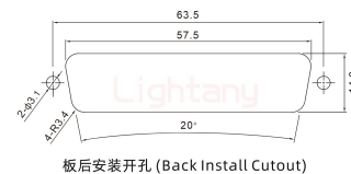
板后安装开孔 (Back Install Cutout)
