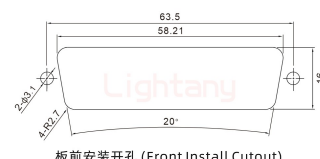
板前安装开孔 (Front Install Cutout)
